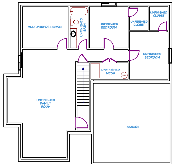
FOUNDATION PLAN
